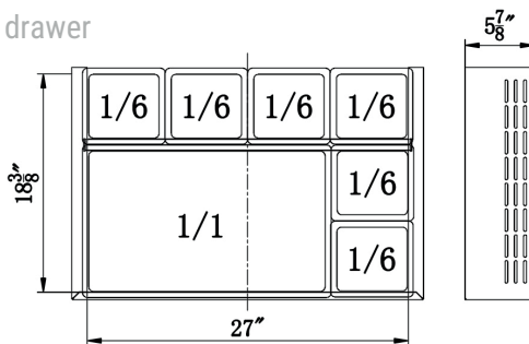
Lower drawer
