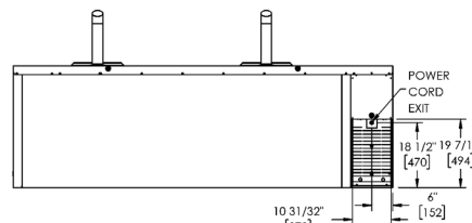
BACK VIEW
